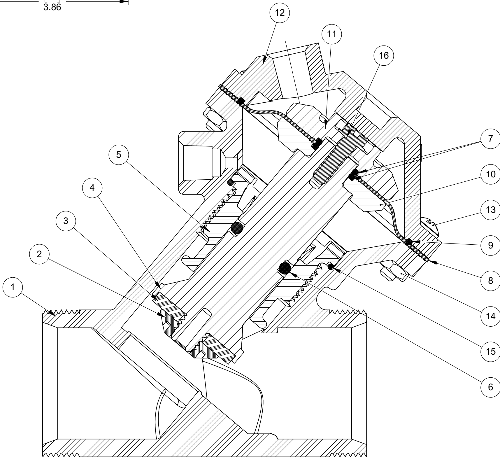
1070154 (K521-X200-14000) NORMALLY OPEN (STANDARD)
