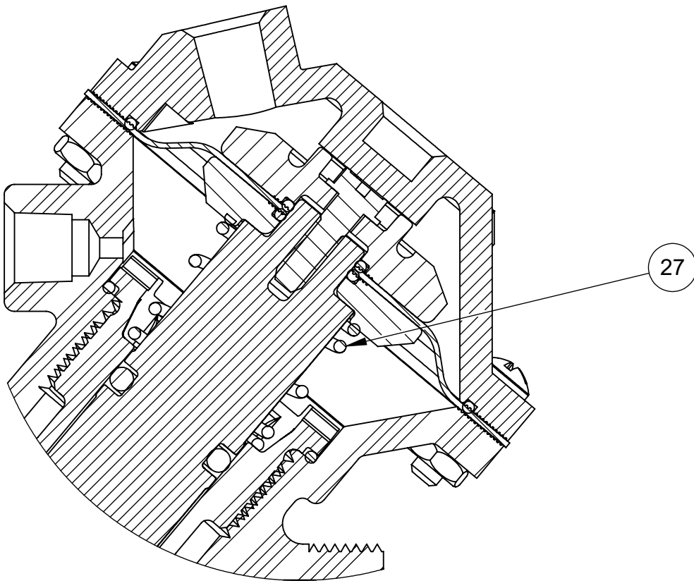
1070158 (K521-X201-14000) SPRING ASSIST OPEN
